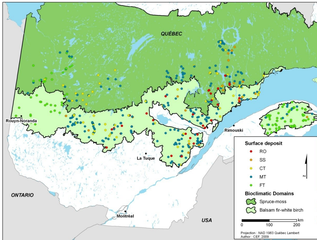
Figure 2.1. Stand location and their respective surface deposit (Abbreviations are as follows: RO, rock outcrop; SS, shallow surface deposit; CT, coarse texture deposit; MT, medium texture deposit; FT, fine texture deposit).
